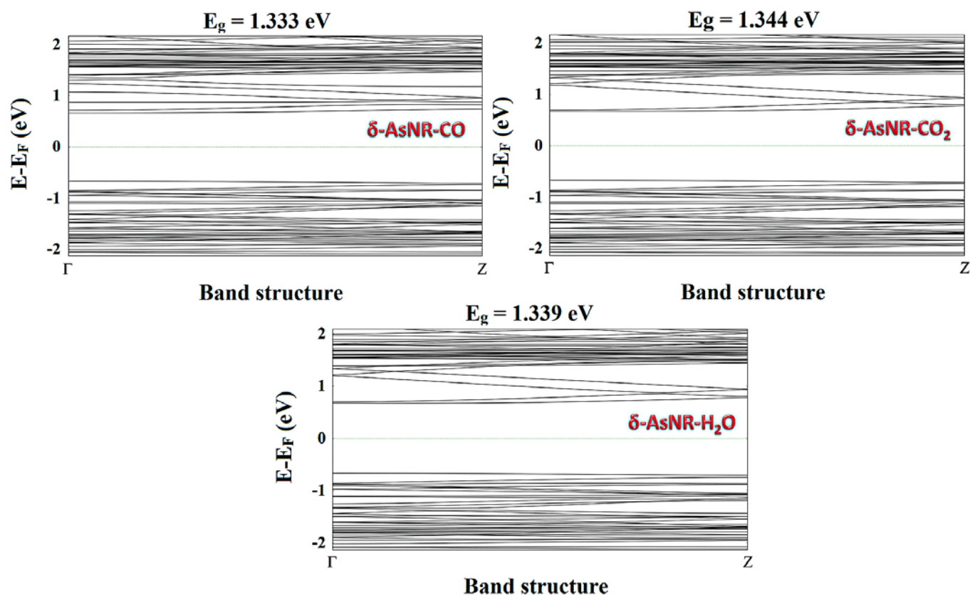
Fig.S1 Band structure of \delta - AsNR with interfering molecules
